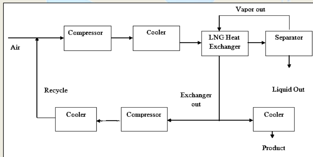
Figure 1: Block diagram of N_2 extraction Process.
